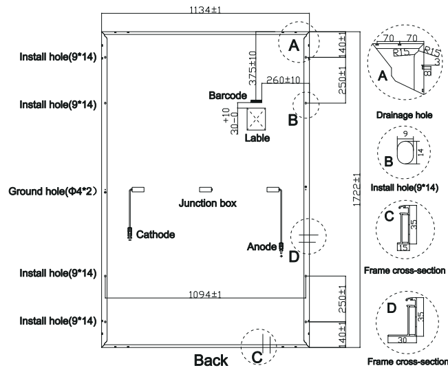
Frame cross-section
